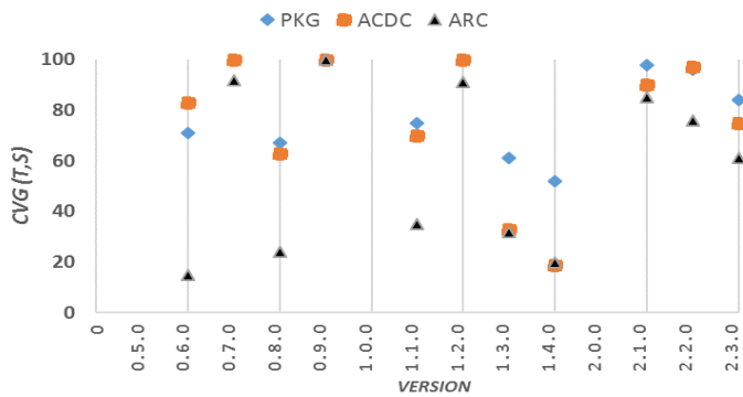
Fig. 14: cvg(t,s) values between minor versions of Ivy
