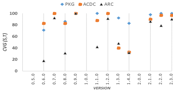
Fig. 13: cvg(s,t) values between minor versions of Ivy
