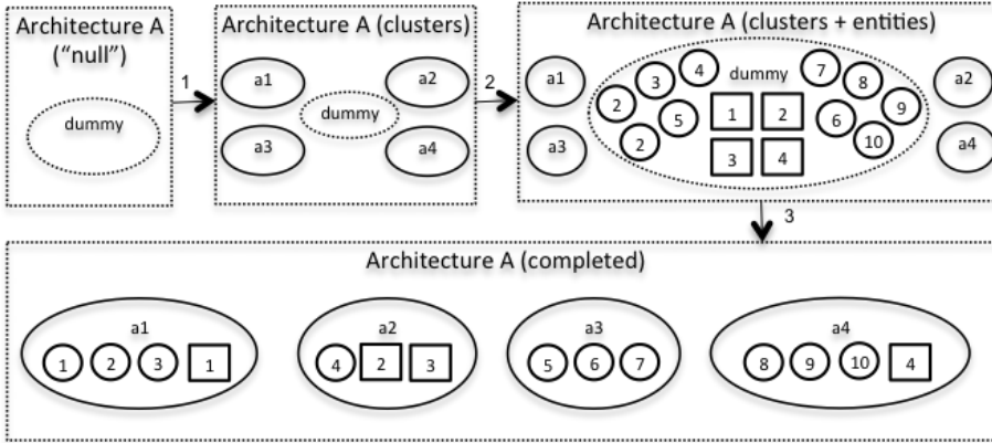
Fig. 2: Constructing architecture A from a “null” architecture: adding (1) clusters and (2) entities, then (3) moving entites into the corresponing clusters.
