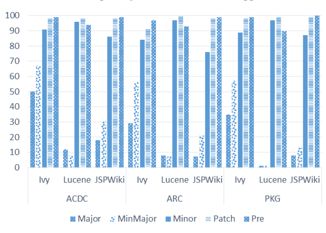
Fig. 11: Average a2a values in three subject systems
