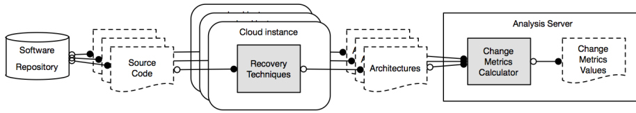
Fig. 10: Deployment of ARCADE components onto the cloud using ARCADE-Controller for rapid, large-scale architecture recovery and analysis.
